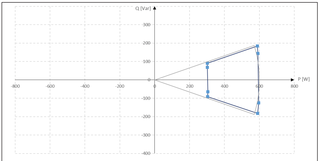
P-Q Diagram
